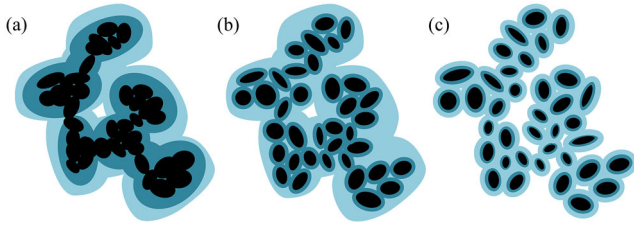
Figure 1. Models of aggregate dust particles. Submicrometre- to micrometre-sized refractory subunits (in black) aggregate to form larger dust particles with sizes on the order of 50–100 \mu\text{m} up to the millimetre scale, typically in a hierarchical fashion, represented here by aggregation of subunits first into units with an intermediate size of 5–10 \mu\text{m} . Three situations are described: (a) if the collision time-scale is shorter than that of ice deposition, subunits first aggregate and subsequently acquire a water ice mantle with a high content of hydrogen halides (dark blue); later, as the halogens have been removed from the gas phase, a pure ice mantle (light blue) is deposited; (b) if the collision time-scale is in between that of halogen-bearing and pure ice deposition, the grains first acquire a halogen-rich mantle before aggregating and then gaining a pure ice envelope. (c) If the collision time is very long, the icy mantles form first and aggregation occurs later on. There must be a smooth transition between these three possibilities. Indeed, the voids between the refractory grains formed in scenario (a) may become filled with halogen-bearing ice after the initial aggregation phase, blurring the distinction with scenario (b). Also, the gradient between halogen-enriched and halogen-poor ice is not so sharp, so that there must be a progressive transition between scenarios (b) and (c) as well. See the main text for more details.
