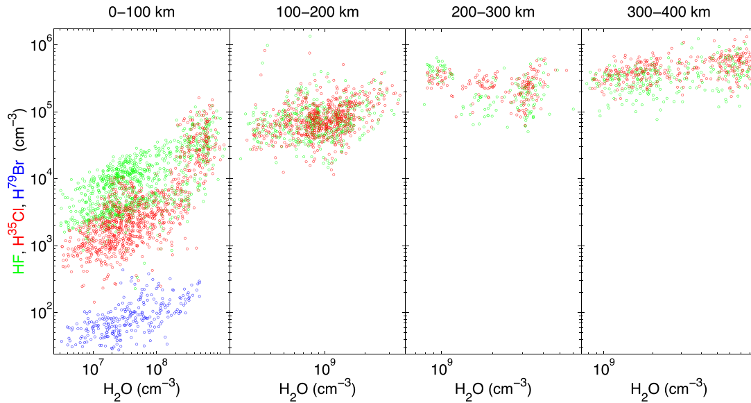
Figure 11. The correlation between HF, HCl, and HBr abundances and \text{H}_2\text{O} changes as a function of spacecraft distance from the comet (corresponding to an increase in comet activity).
