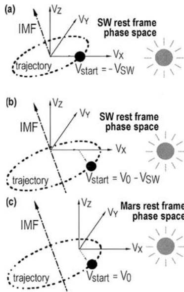
Figure 4. Illustration of ion motion in the solar wind ( \mathbf{V}_{SW} ) with respect to the IMF in a velocity space diagram ( V_X, V_Y, V_Z ) where X, Y, Z directions are given in Figure 1. (a) An ion with zero initial speed (i.e., negligible compared to the solar wind velocity) in the Martian rest frame has an initial velocity of -V_{SW} in the solar wind frame. Since there is no electric field in the solar wind frame, the ion performs a simple spiral motion around the IMF (the magnetic field direction is about the same in both the Martian rest frame and the solar wind frame). Any spiral motion is represented by a circle about the magnetic field in velocity space. (b) For the finite initial velocity ( \mathbf{V}_0 ) in the Martian rest frame, the start position is shifted by \mathbf{V}_0 from (a), and hence the radius of the ring changes. However, the ring is still found around the IMF and the ion speed (distance from the origin of coordinates) is constant. (c) The Martian rest frame trajectory of what is shown in (b). The difference between (b) and (c) is only a constant velocity +V_{SW} .
