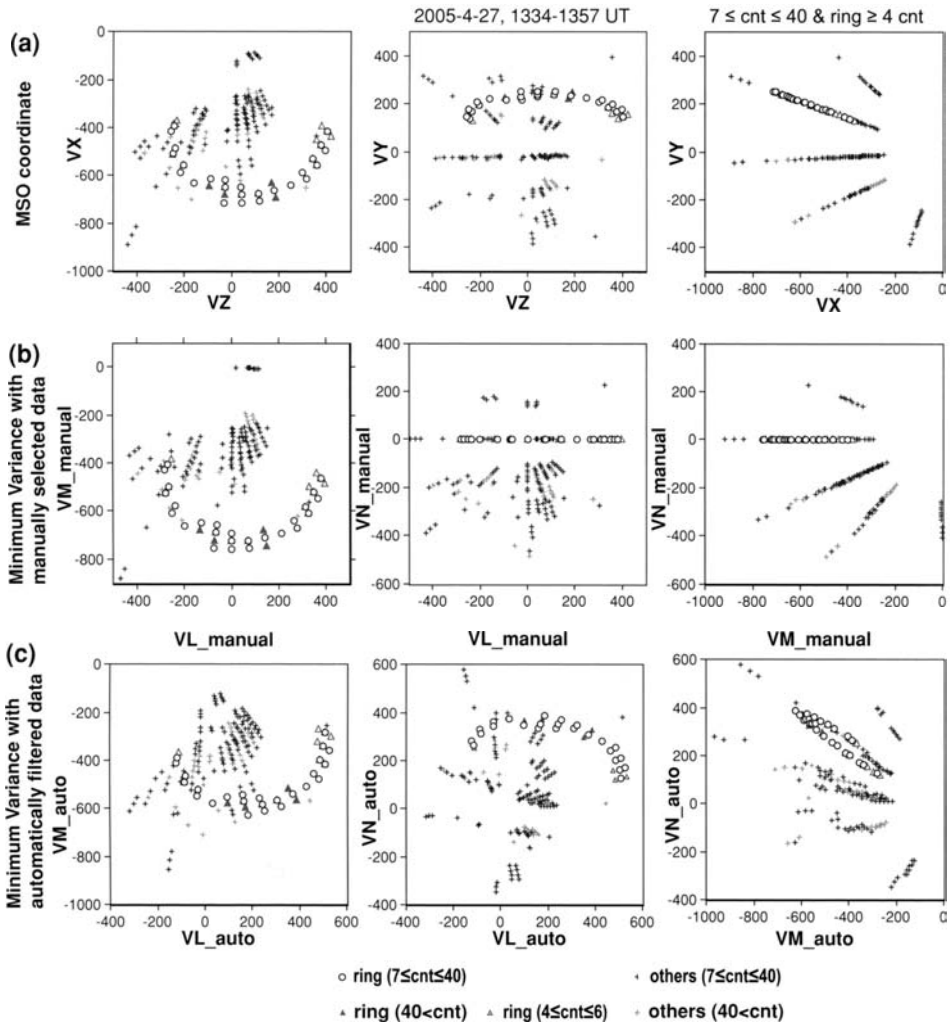
Figure 5. Velocity scatter plots of the ion data (all axes are in km/s) during 1334–1357 UT, 27 April 2005, in (a) MSO coordinates, (b) local LMN (minimum variance) coordinates determined from Table I (manual method) and (c) local LMN coordinates determined from automatically filtered data during 1337–1357 UT. The selected data are ion mass range 0.5–1.1 (proton channel: it is slightly contaminated by the solar wind alpha particles as seen in Figure 2). Plotted data consist of points that have more than 3 counts and azimuth = 0 data are not shown (total 450 points). The circles and triangles denote to the point belong to the ring distribution by a manual inspection, with circle corresponding to 7–40 counts, filled triangle corresponding to more than 40 counts, and empty triangle corresponding to 4–6 counts. Non-ring data are shown using plus marks (black: count is 7–40, grey: count more than 40).
