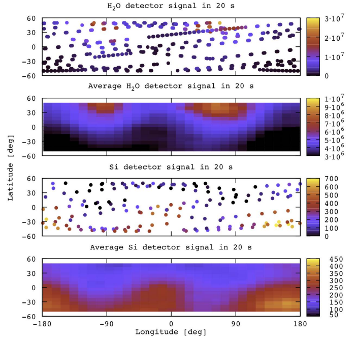
Fig. 3. Maps for the H 2 O (top two panels) and the Si signal (bottom two panels) measured with DFMS. Top panel and third panel from the top: actual measurements, normalized onto a 10 km sphere around the nucleus. Other two panels: interpolation of these signals to a complete map.
