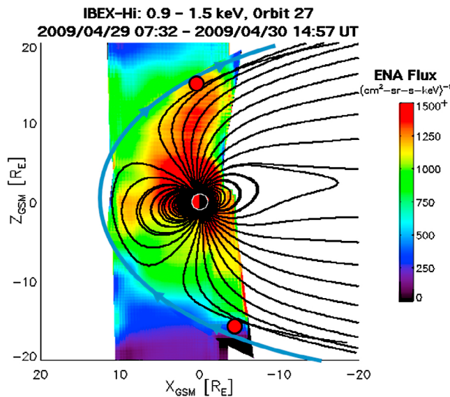
Figure 6. An ENA composite image of the cusps, during northward IMF conditions. Overlaid is the draped magnetosheath magnetic field (blue), marking the locations just tailward of the cusps where magnetic reconnection is likely to occur (red circles).
