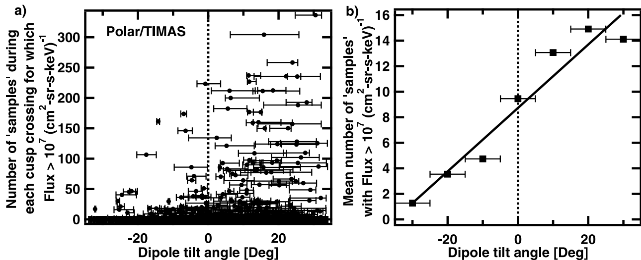
Figure 4. (a) Time intervals during each Polar pass through the northern cusp for which the number flux at E = 1 keV is >10^7 ( \text{cm}^2 \text{ sr s keV}^{-1} ). (b) The mean number of time intervals within each 10^\circ dipole tilt angle bin.
