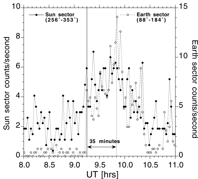
Figure 1. LENA total atom rates (single spin, 120 sec accumulations) from the sun sector (left y axis) and from the Earth sector (right y axis) vs. time for the 8 June 2000 CME event.
