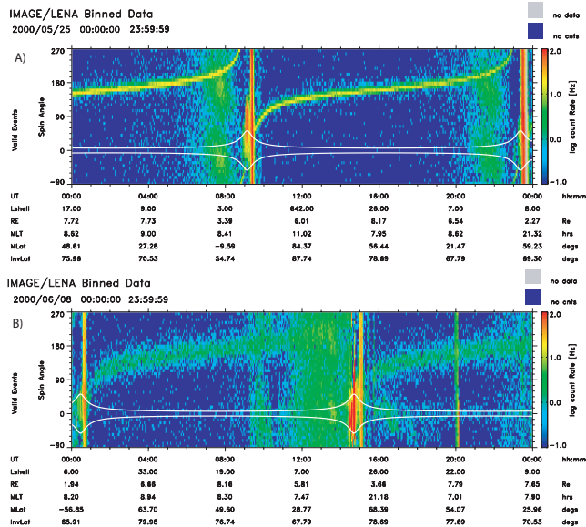
Plate 1. LENA total atoms (coincidence) spin spectrogram for A) the period of 25 May 2000, and B) for the CME event of 8 June 2000. Spin angle increases with time, with reference (0) to the nadir view. White lines indicate the limbs of the Earth.
