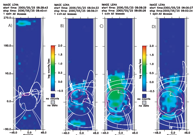
Plate 2. LENA image sequence for 25 May 2000; A) during downleg just past descending node, sun at top; B) approaching passage over the south polar regions, sun at lower left; C) passing over the Antarctica; and D) near perigee, with sun near occultation. Each image contains the Earth with continents, nominal auroral oval in red, and 3 and 6.6 R_E magnetic field lines at the indicated magnetic local times.
