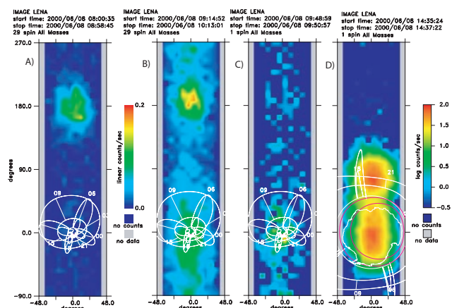
Plate 3. LENA image sequence for 8 June 2000; A) hour average before CME arrival at 0915; B) hour average after CME arrival; C) snapshot 35 min after CME arrival; D) passage over the south polar regions near perigee. Panels A, B, C have linear scaling (color bar C 10x higher than for A, B), whereas D is logarithmic.
