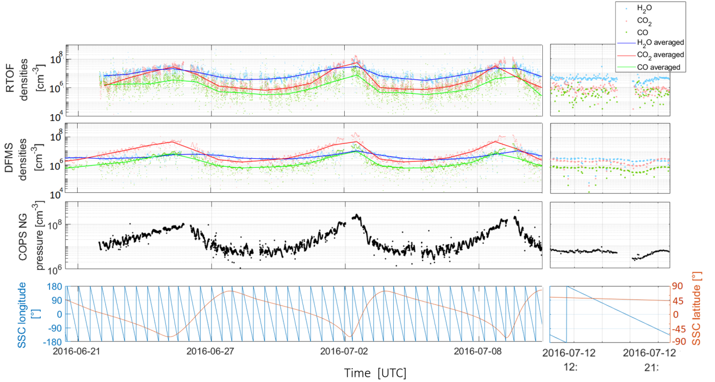
Fig. 3. Left: temporal evolution after equinox of the densities of the RTOF ( first panel ) and DFMS main volatiles ( second panel ) with the average over two comet rotations (colored lines), the COPS nude gauge total densities ( third panel ), and the SSC point latitude and longitude ( fourth panel ). Right: zoom-in on one rotation (~12 h).
