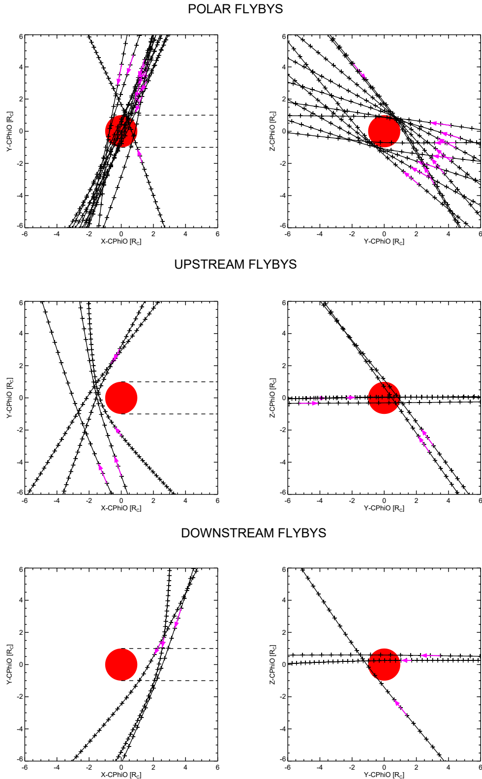
Figure 3. The Callisto flybys categorized in terms of plasma configuration in 12 polar (top), 5 upstream (middle), and 3 downstream (bottom panel) flybys, plotted in the xy -plane (left column) and the yz -plane (right column) of the Corotation-Jupiter reference frame. In this reference system, the local plasma corotation direction points to +X , Jupiter is at +Y , and +Z closes the right-handed system. The position of Callisto's plasma wake is indicated in the xy -plane, the pink arrows indicate the spacecraft direction.
