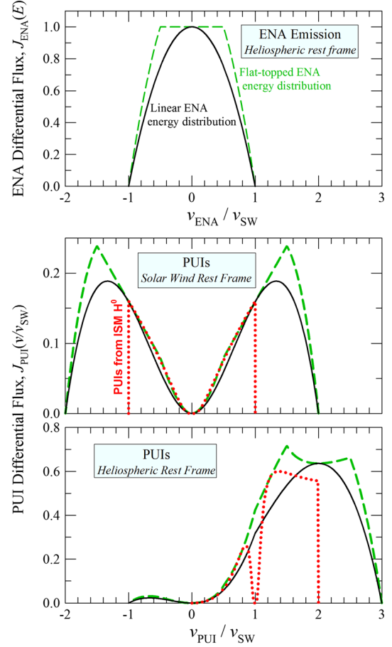
Figure 13. Ionized ENAs from the Moon or interplanetary dust with initial flux distributions (top) are injected gyrotronically into the solar wind, resulting in a filled shell distribution of pickup ions (PUIs) in the rest frame of the solar wind (middle). A negative value of v/v_{SW} corresponds to a direction back toward the Sun. Transforming this PUI distribution into the heliospheric rest frame yields the differential flux (bottom). The dashed green and solid black lines correspond to the linear and flat-topped ENA injection energy distributions used in Figures 10 and 12. The flat-topped distribution for Figure 13 uses a flat ENA emission flux up to 0.5v_{SW} , which corresponds to E_T = 0.25 keV and E_{SW} = 1 keV. As explained in Figure 10, the linear approximation applies when v_{SW} equals or exceeds the fast solar wind speed. The PUI flux in the bottom panel is characteristic of what might be observed downstream of an extended scattering source such as interplanetary dust due to reflected solar wind protons. The red dotted line corresponds to the characteristic flux distribution resulting from ionization of cold interstellar neutral atoms that travel to the inner heliosphere.
