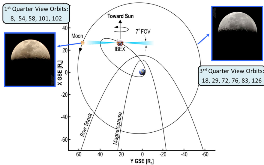
Figure 1. Because of its orbit and viewing geometry (a circular swath in a plane perpendicular to its Sun-pointed spin axis), IBEX observes a portion of the Moon illuminated by the solar wind that is nearly identical to the sunlit portions of the first or third quarter Moons.
