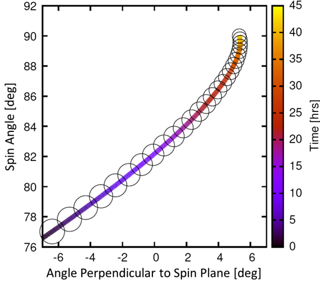
Figure 3. The transit of the Moon as viewed at IBEX throughout the encounter of IBEX Orbit 83. The spin angle is the angle of the circular swath observed by IBEX each spin throughout an IBEX orbit; a spin angle of 0^\circ corresponds to ecliptic north. The single pixel FOV of IBEX-Hi has an angular resolution 13^\circ full width at full maximum (FWFM), which is the extent of the horizontal axis (angle perpendicular to the spin plane). The circles qualitatively represent the angular size of the lunar disk at IBEX at regular 1.53 h intervals throughout the \sim 45 h encounter, over which statistically significant counts were obtained for \sim 25 h. The IBEX-Moon geometry can be complex and variable, but it is accurately determined using knowledge of the IBEX location and spin axis vector.
