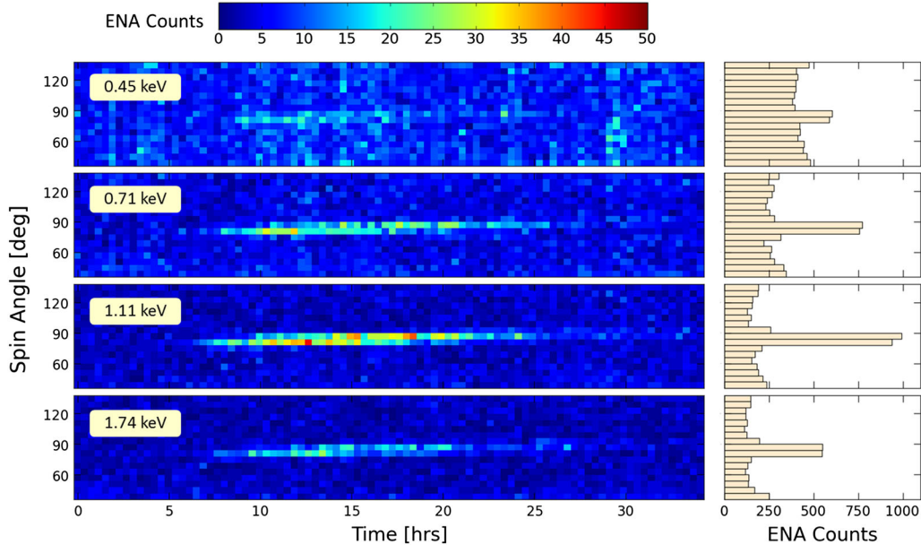
Figure 4. Lunar observation during IBEX Orbit 83 for the four lowest energy passbands of IBEX-Hi. Color histograms are the number of counts as a function of spin angle \theta (binned to 6^\circ ) and time. Each time bin corresponds to 96 spins ( \sim 0.383 h) although quantitative analysis of the ENA counts is performed over time bins of 1.53 h for statistical significance. Spin angles of 0^\circ and 180^\circ correspond to ecliptic north and south, respectively. The plot to the right of each color histogram is the total number of counts for each spin bin acquired over the interval 6–27 h. The lunar signal lies near \theta = 90^\circ in all plots.
