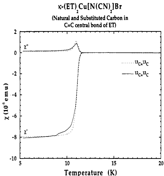
Figure 1. Superconducting transition, as determined by ac susceptibility measurements, of \kappa\text{-(ET)}_2\text{Cu[N(CN)}_2\text{]Br} with normal ^{12}\text{C}=^{12}\text{C} and with ^{13}\text{C}=^{13}\text{C} labeling in the central double-bonded carbon atoms of ET. The symbols \chi' and \chi'' refer to the real (in-phase) and imaginary components, respectively, of the total susceptibility. The mean-field superconducting transition temperatures ( T_c ) are 11.42 \pm 0.05 K for the ^{12}\text{C}=^{12}\text{C} crystal and 11.43 \pm 0.04 K for the ^{13}\text{C}=^{13}\text{C} crystal.
