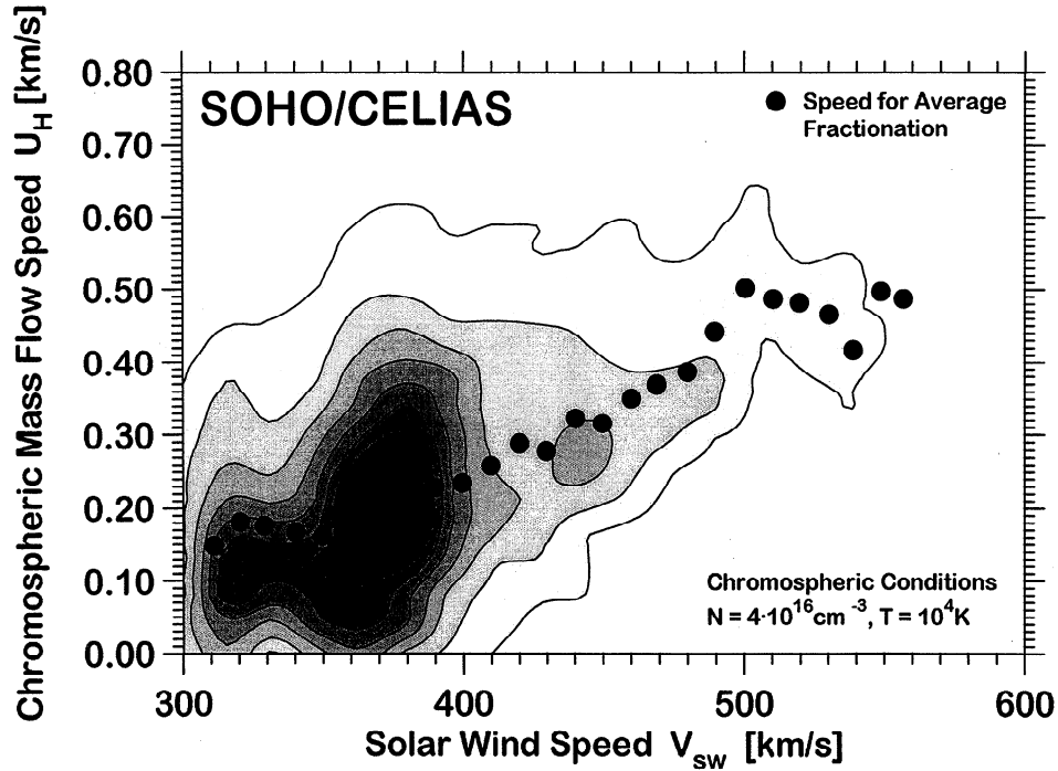
Figure 8. Contour plot (linearly spaced) of the chromospheric mass flow speed U_H and the solar wind bulk speed v_{sw} for the entire time period analyzed. The speed U_H was derived from the observed fractionation factors f_{Fe,O} using (1). Correspondingly, from the average values of \log(Fe/O) within speed bins 10 km/s wide, average values of U_H for the same bins of the solar wind speed were derived (dots).
