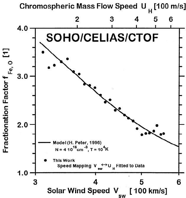
Figure 9. Speed dependence of the fractionation factor f_{Fe,O} . The modeled fractionation (solid line) depends on the chromospheric mass flow speed U_H (top axis) according to (1). The mapping between U_H and the solar wind proton speed v_{sw} (equation (2)) was fitted to match the average fractionation factors derived from the data (dots).
