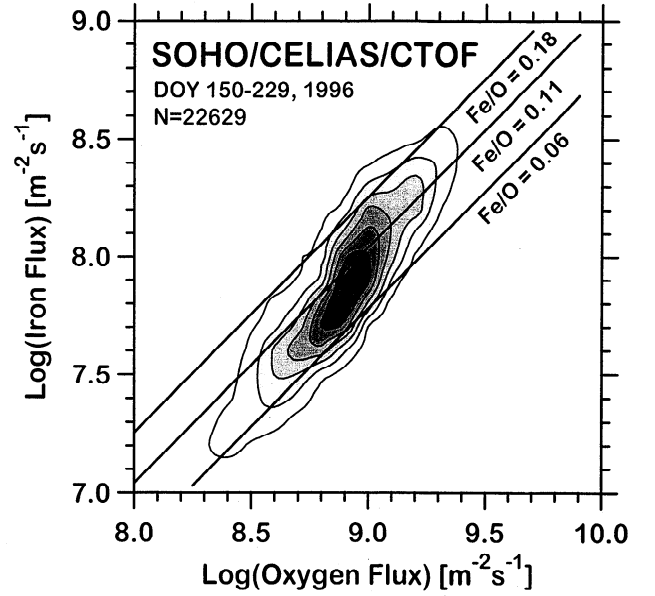
Figure 2. Correlation of the iron flux and the oxygen flux in the solar wind. The three solid lines represent cases of a constant flux ratio of Fe/O of 0.06, 0.11, and 0.18, respectively. The Fe/O ratio is not constant in all solar wind regimes and increases with increasing flux of oxygen. Data were taken between day of year (DOY) 150, 1996, and DOY 229. N denotes the number of spectra processed.
