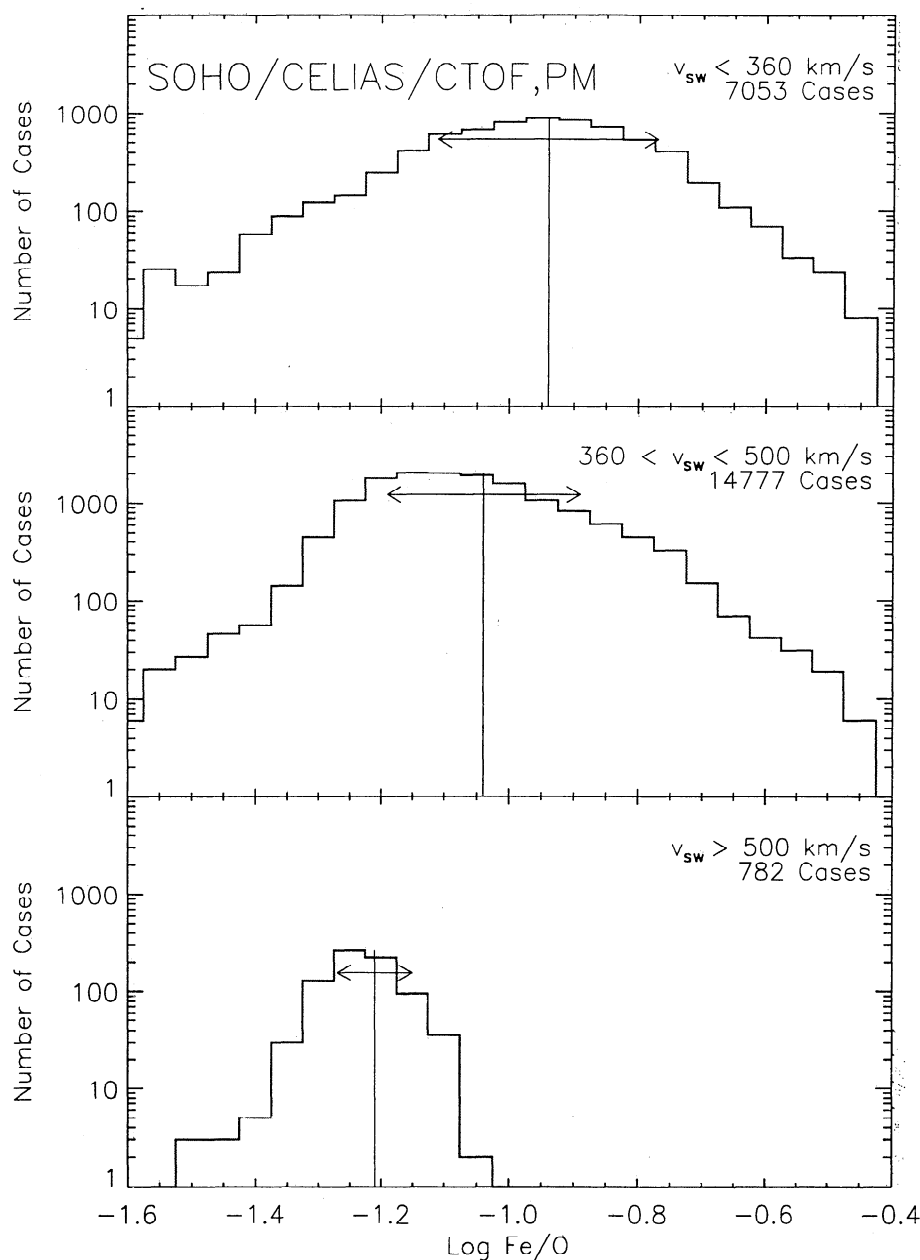
Figure 3. Histograms of \log \text{Fe/O} for three different ranges of the solar wind speed v_{sw} . In each histogram the vertical line indicates the mean value, and the horizontal arrows give the standard deviation of the sample. The cases in the highest speed range were accumulated during four distinct periods which are separated at least by 10 days.
